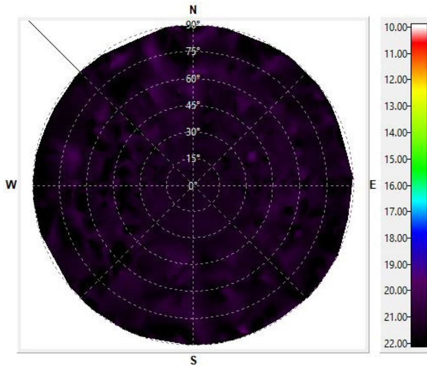
Figure 4.1: Light 1 Sky Brightness Plot, Comprised of 12 Sampling Events (mag/arcsec 2 )
