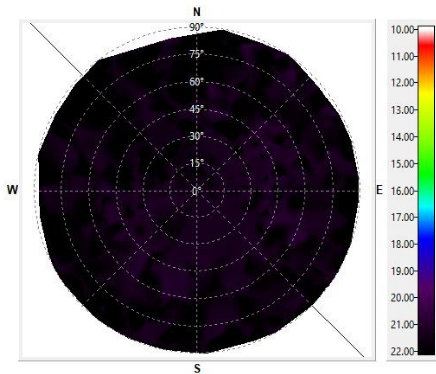
Figure 4.4: Light 4 Sky Brightness Plot, Comprised of 8 Sampling Events (mag/arcsec 2 )
