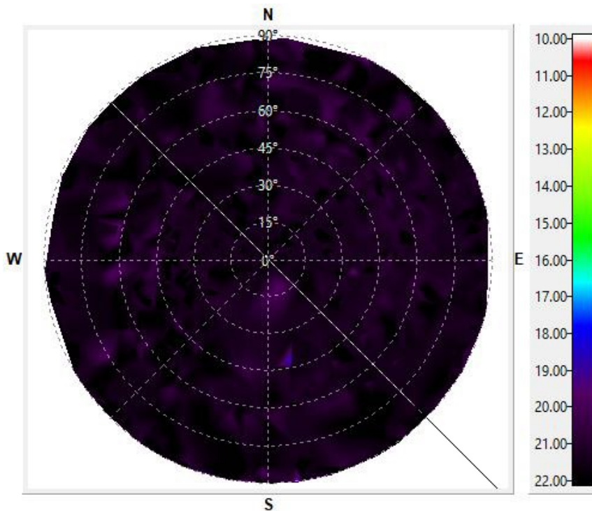
Figure 4.2: Light 2 Sky Brightness Plot, Comprised of 12 Sampling Events (mag/arcsec 2 )
