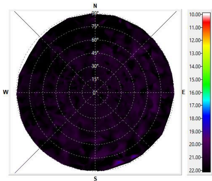
Figure 4.3: Light 3 Sky Brightness Plot, Comprised of 12 Sampling Events (mag/arcsec 2 )
