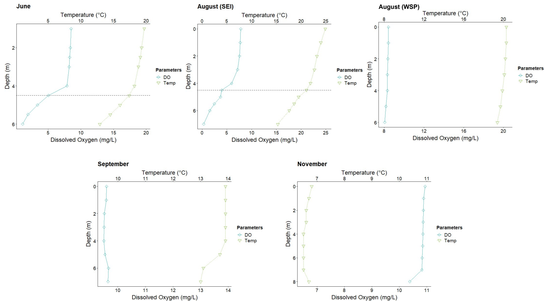
Plate A1-3: York Lake Temperature-DO Profiles (2021)
