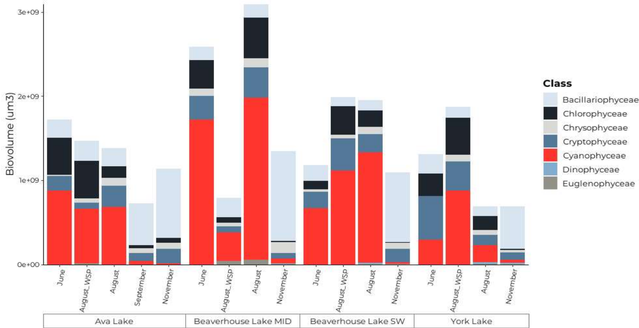
Figure D1-3: Total Phytoplankton Biovolume (um 3 ) by Taxonomic Group and Lake 2021
